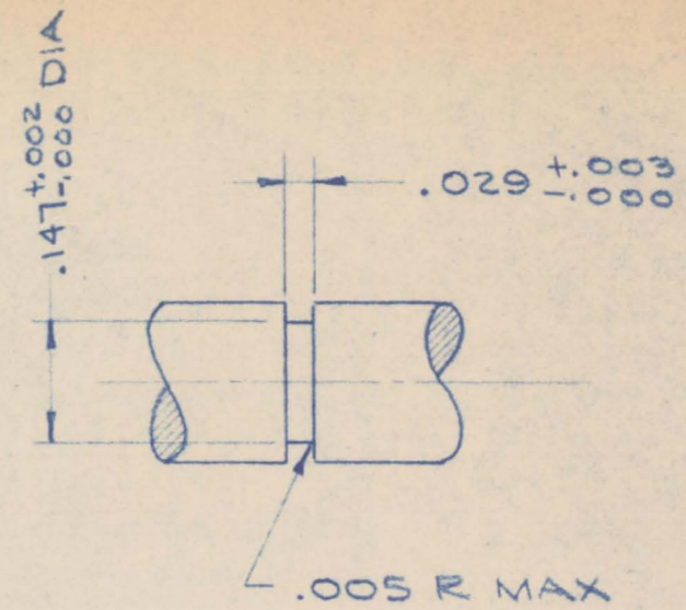
DETAIL "A" RING GROOVE FOUR TIMES SIZE
